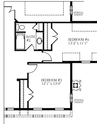
PARTIAL UPPER LEVEL PLAN with optional 8' side extension
